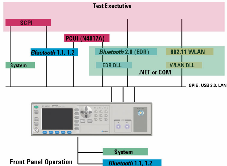
Figure 1-1 N4010A Interfaces and DLLs Rear Panel Operation
